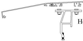
Aluminum Hood
